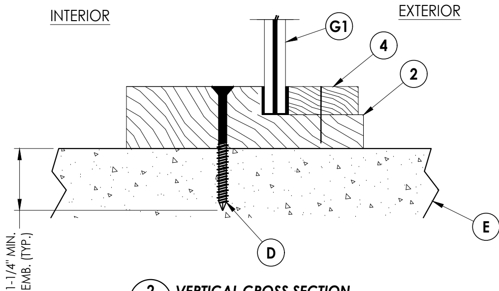
2 5 VERTICAL CROSS SECTION
