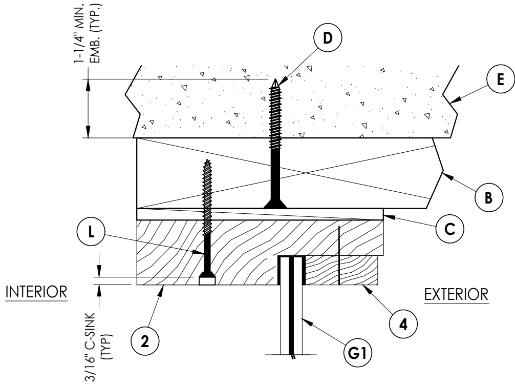
1 5 VERTICAL CROSS SECTION
