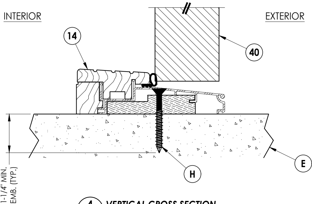
4 5 VERTICAL CROSS SECTION
