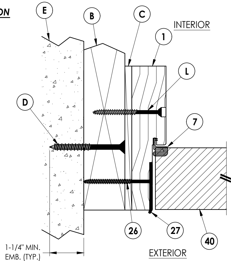
4 6 HORIZONTAL CROSS SECTION
