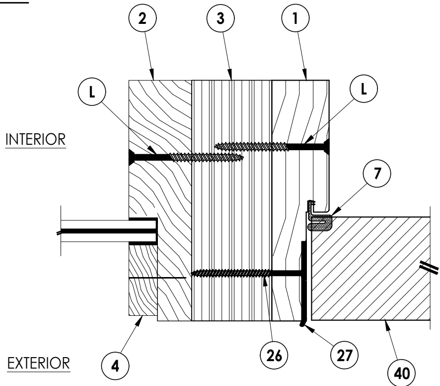
2 6 HORIZONTAL CROSS SECTION
