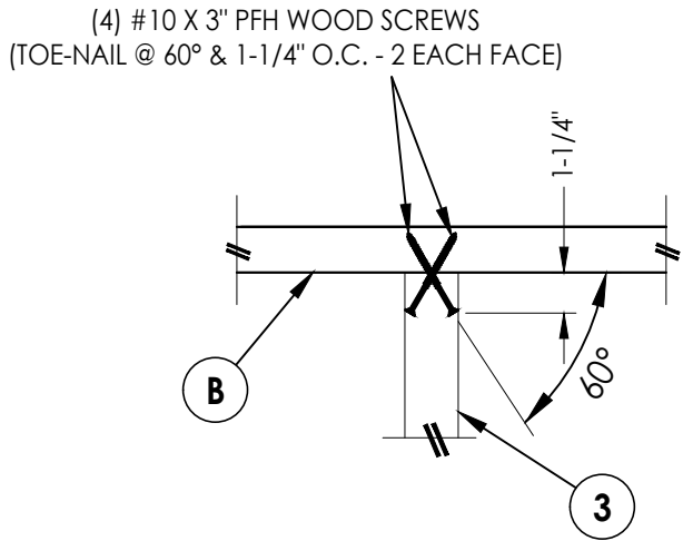
MULLION-TO-HEAD CONNECTION DETAIL
