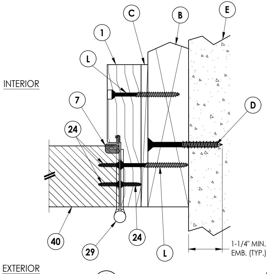
3 6 HORIZONTAL CROSS SECTION
